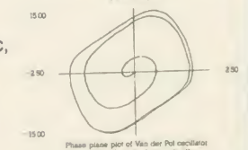
Phase plane plot of Van der Pol oscillator (mu = 4, horizontal, x, vertical)
